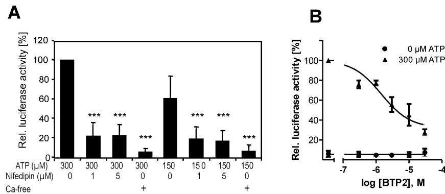
Figure 4 \text{Ca}^{2+} channel blockers inhibit ATP-induced NFAT activation. A , Effect of nifedipine and dependence on extracellular calcium. PC12-NFAT-Luc cells were treated for 3 h with ATP and nifedipine as indicated or were stimulated with ATP in the absence of extracellular free \text{Ca}^{2+} . Nominal \text{Ca}^{2+} -free conditions were created using 2 mM EGTA. Statistical significance is indicated for differences vs. the control cells treated only with 300 \mu\text{M} ATP or 150 \mu\text{M} ATP ***, p < 0.001 . B , Effect of BTP2. Cells were treated with varying concentrations of BTP2 during ATP stimulation. A simple inhibitor-response curve was tentatively fitted to the data, although more than one mechanism may contribute to the inhibitory effect of BTP2. The calculated \text{IC}_{50} is 1.5 \mu\text{M} (95% confidence interval 0.7-3.3 \mu\text{M} ). Luciferase activities are expressed as the fold stimulation by the treatment relative to that in cells only treated with 300 \mu\text{M} ATP. Both graphs show means \pm SD of 3 independent experiments.
