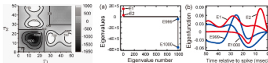
Figure. 1 left: STC of the rat hippocampal CA1 pyramidal neuron. (a) Eigenvalue spectrum of \Delta C for the same neuron as illustrated in the left panel. (b) Excitatory (red) and suppressive (blue) eigenfunctions corresponding to the eigenvalues in (a).
