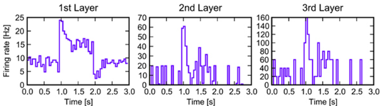
Figure 1 Layer-specific population response in a simplified feed-forward network of the insect olfactory pathway. Average population response in the first layer (left) to a step-like Poisson input shows a phasic-tonic response as observed in antennal lobe projection neurons. In the second layer (middle) the population response profile is dominated by a sharp onset transient and tonic firing is diminished. The final output layer (right) with reduced adaptation current integrates convergent input.
